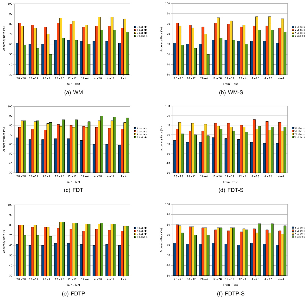
Fig. 11. Comparison of the selected rule induction methods regarding test data. (a) WM, (b) WM-S, (c) FDT, (d) FDT-S, (e) FDTP, and (f) FDTP-S.
