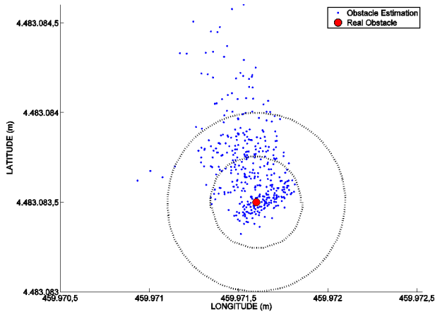
Figure 8. Blue dots represent obstacle location estimation during the real tests and the red dot represents the real position of the obstacle. The mean error is 49 centimetres and a circular grid of 0.5 metres is displayed around the obstacle to show the error of each estimation.
