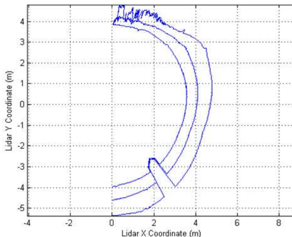
Figure 4. Representation of three LIDAR layers in the presence of an obstacle. The continuous smooth projection of LIDAR measurements is broken in presence of an obstacle.
